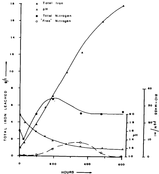
Fig.2. A leach test on the Tharsis pyrite (-45 \mu\text{m} ) at 6% pulp density indicating the bio-mass present. Initial pH 2.0, temperature 35°C.
