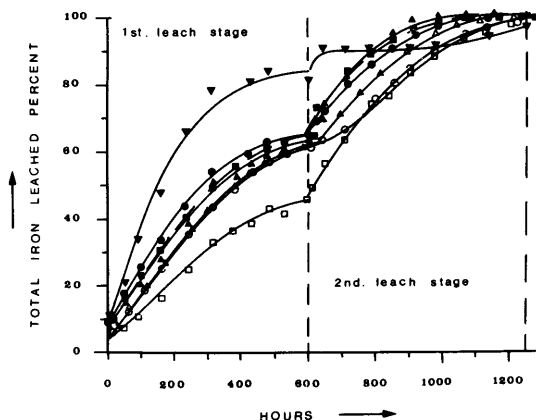
Fig.3. Two stage bacterial leach profile of pyrite samples from various geological origins. Pulp density 6%, temperature 35°C, initial pH 2.0.
