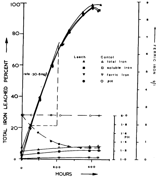
Fig.1. A typical leach test on a 2% pulp density Tharsis pyrite (-45 µm) Temperature 35°C, initial pH 2.0.
