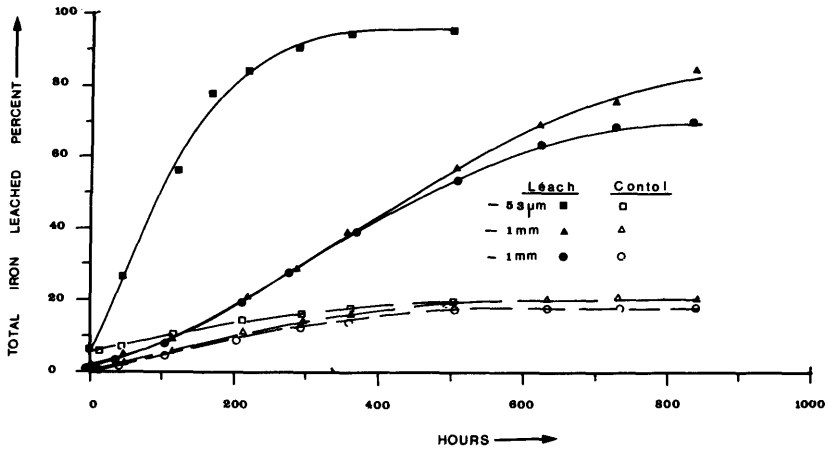
Fig.6. Bacterial leaching tests on the Amman Rider Coal samples of various size fractions. (Δ Sieved 0 Crushed). Pulp density 10%, temperature 35°C, initial pH 2.0.
